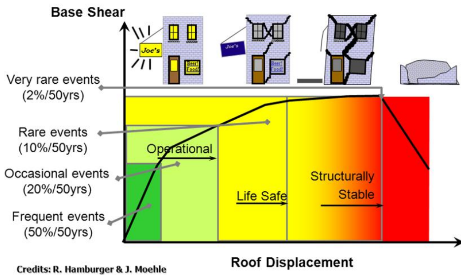
Figure 8: Anatomy of a static pushover curve
