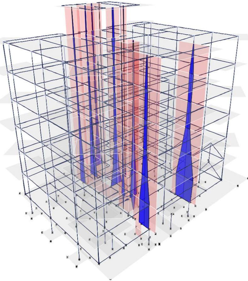
Figure 5: Pier Element main moment Range under U.L.S. Earthquake Combination in main X-direction.
