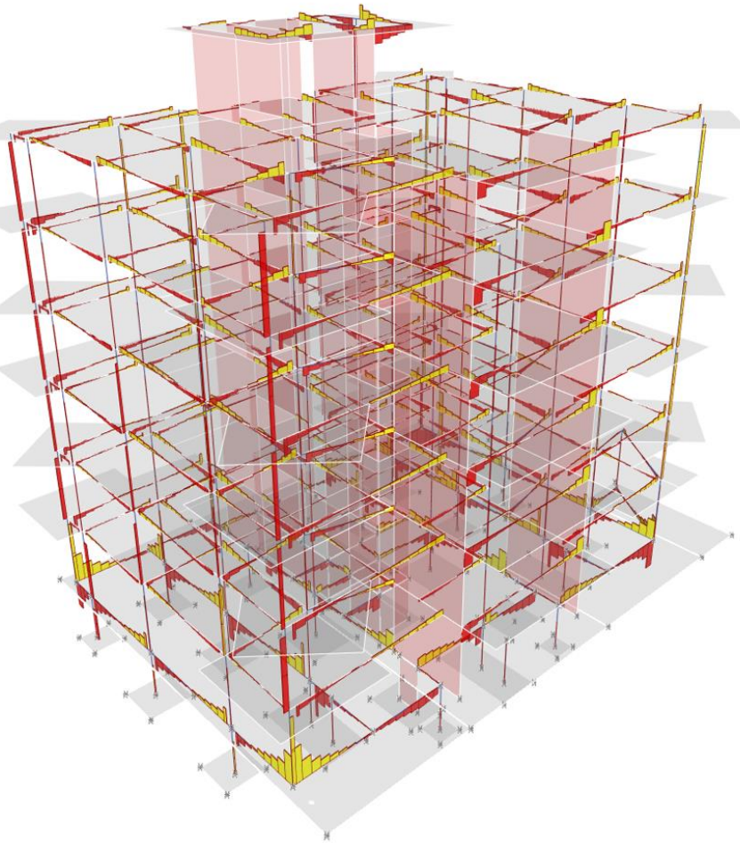
Figure 7: Frame Element main shears under U.L.S. combination 1.35G + 1.5Q.
